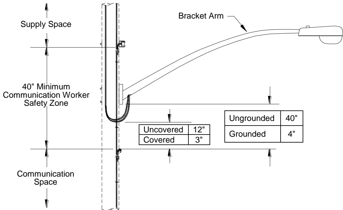
Figure 11 Clearances for Street Light Above Communications
