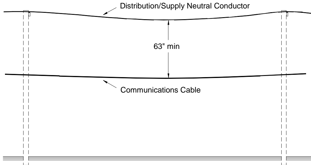
Midspan Clearance between Distribution Conductors and Communications Cables
