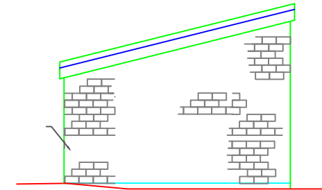
NORTH ELEVATION
