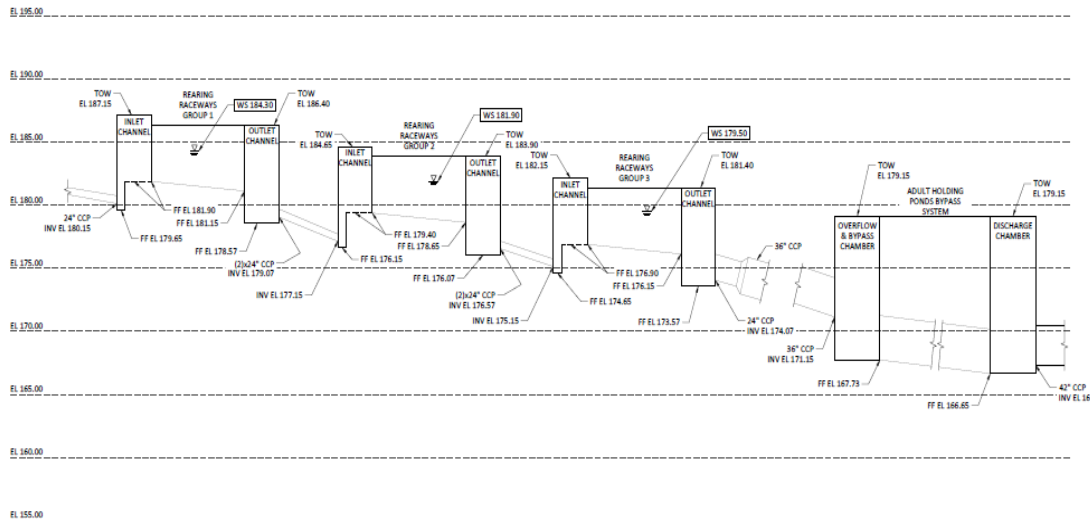
1 001 COWLITZ TROUT HATCHERY HYDRAULIC PROFILE REARING RACEWAYS GROUP 1, 2, & 3, ADULT HOLDING PONDS BYPASS SYSTEM SCALE: NTS
